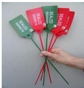
Art: RFID TITAN SEAL Plastic seal. Flat tail with spikes. Ink transfer print 5x328 mm 5x424 mm Label: 72x110mm RFID UHF -HF/NFC seal
