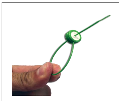
Art: MEROPE SEAL Plastic seal with metal closure. Round and smooth tail. Laser print. 1x 161 mm
